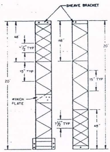
SECT. 5 SECT. 3 & 4 BRACE CONFIGURATION
