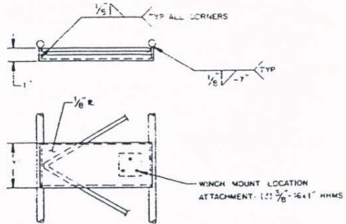
WINCH MTG. PLATE
